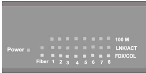
Figure 2-4. LED Indicators
